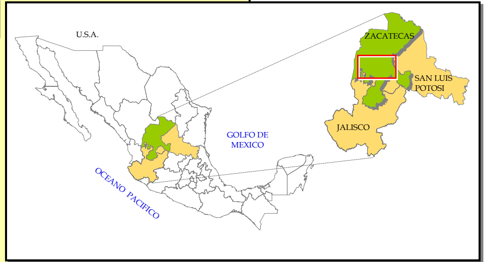
Fig. 7: ZACATECAS GEOLOGY & SYSTEMS
