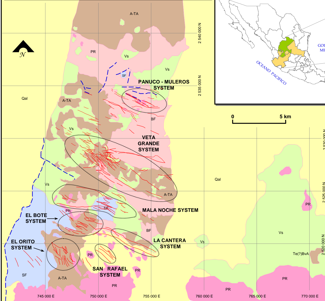
Fig. 7: ZACATECAS GEOLOGY & SYSTEMS
